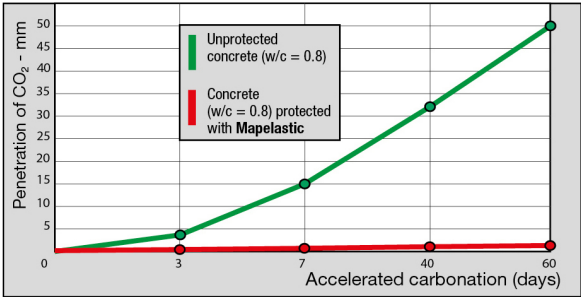
Fig. 2: Protection of Mapelastic against accelerated carbonation (30% of \text{CO}_2 ) on porous concrete
