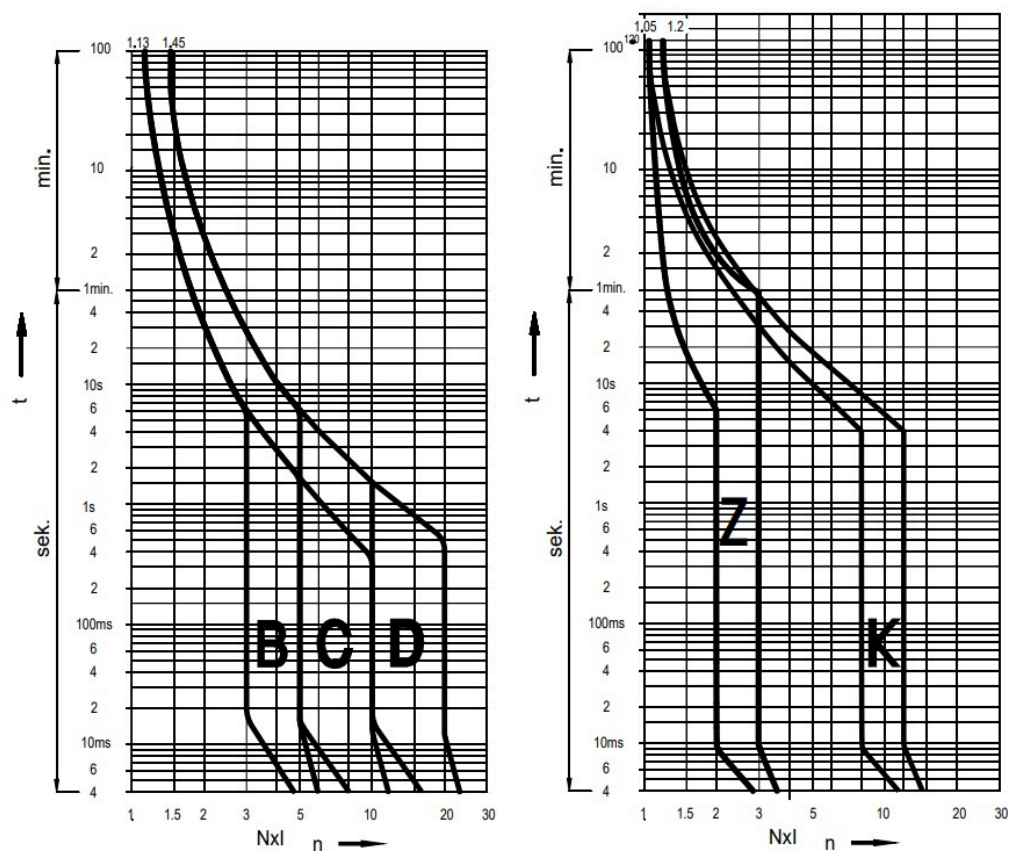
I/t characteristic at 50 and 60Hz
