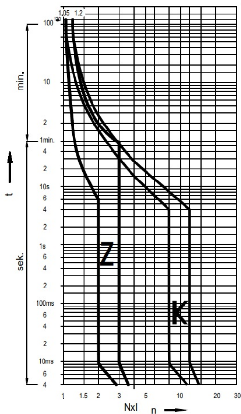
I/t characteristic at 50 and 60Hz
