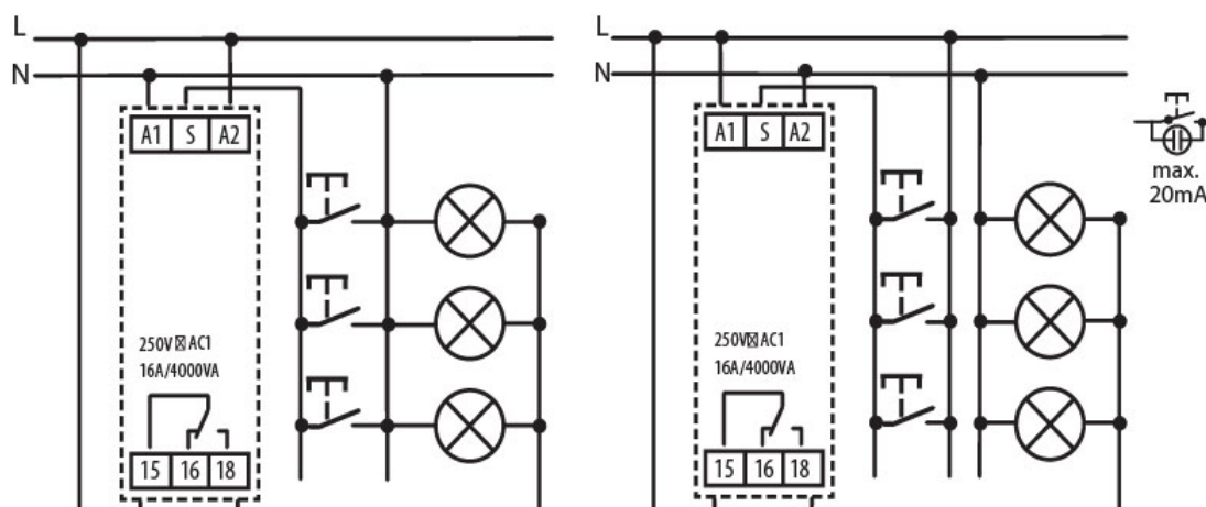
3-wire connection
